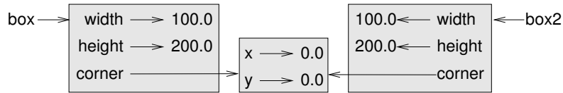
Figure 15.3: Object diagram.
